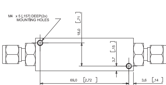
Figure 6 Dimensions for 4800 Series Devices with Standard Process Connections
