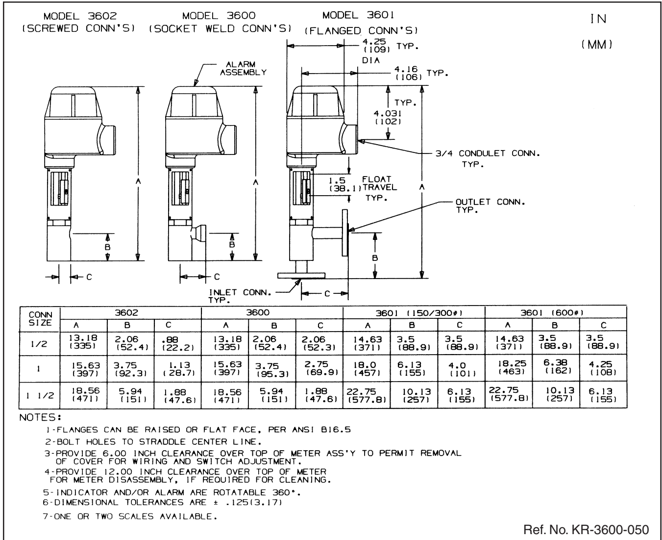
Figure 2 MT3600 Series Meter with Alarm Dimensions
