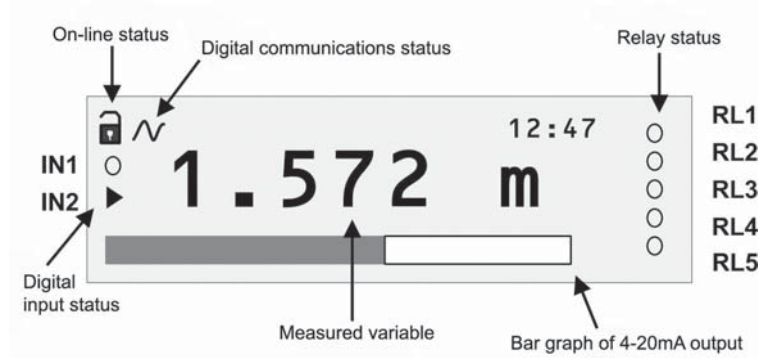
4 line display
