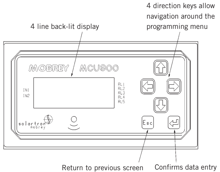
Display and keypad
