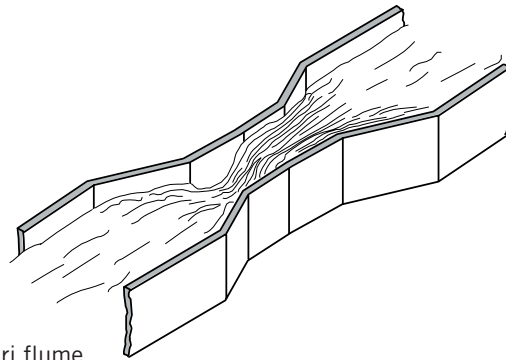
Venturi flume Typical 3/2 power law
