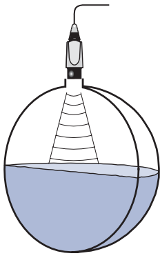
Spherical tank
